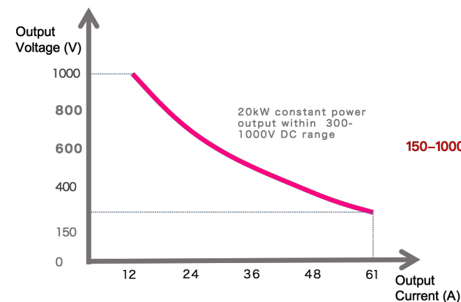
Constant power output range curve
